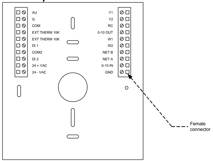
Thermostat's baseplate
